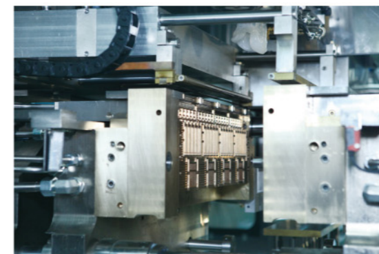
小容量容器产品模具 Small Volume Product Mould
